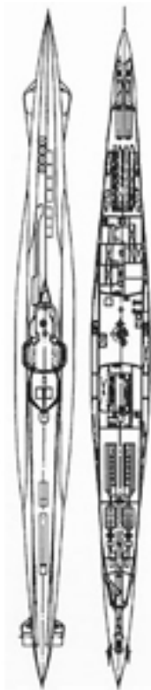
Type VIIC U-boat
